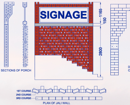
DETAIL OF CORBEL
