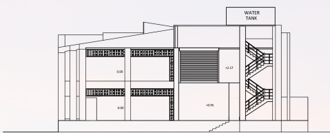
WEST ELEVATION
