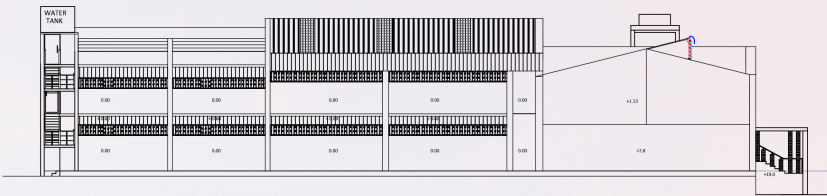
SOUTH ELEVATION
